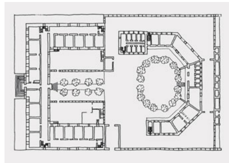
015 Walnutstreet Jail Philadelphia (1790)
