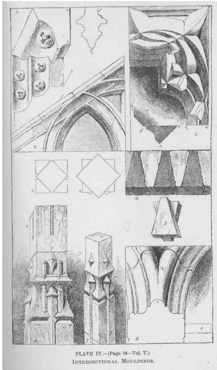
PLATE IV.—(Page 66—Vol. V.) INTERSECTIONAL MOULDINGS.
