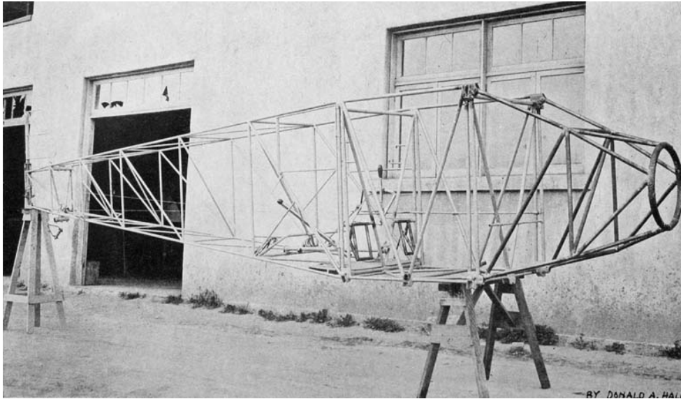
Fuselage frame of the plane
