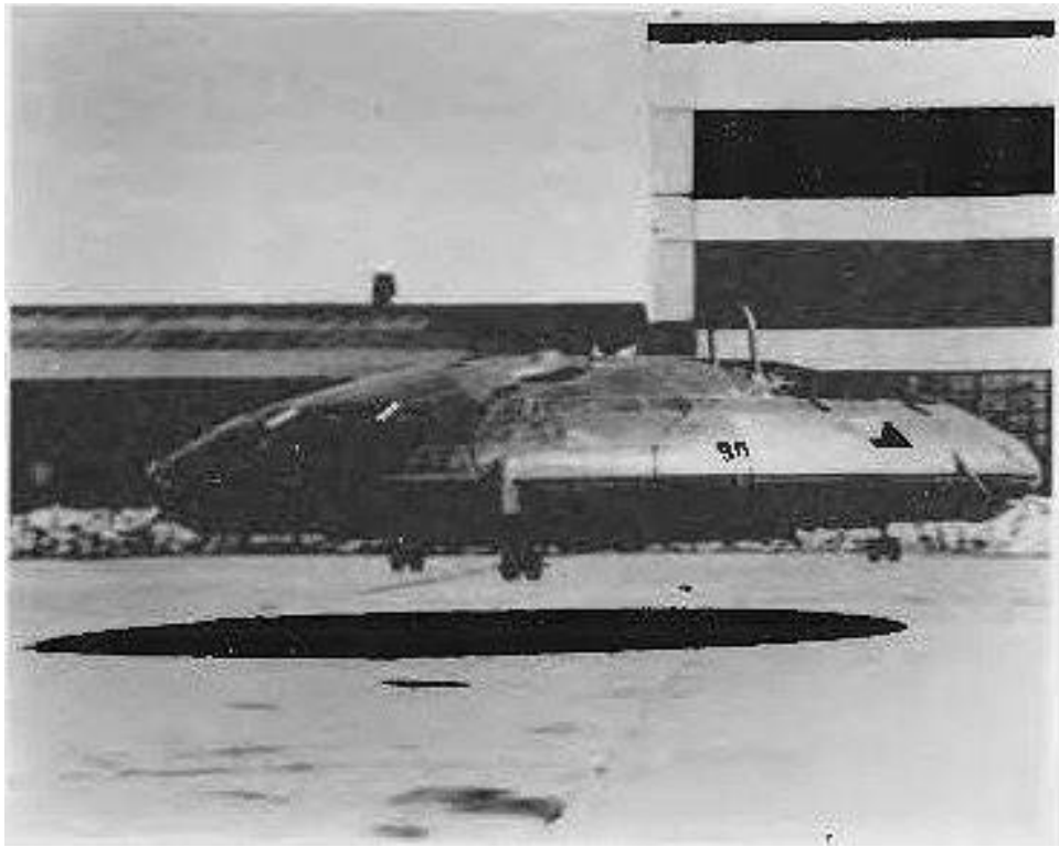
Avro Canada VZ9 Avrocar. Photo US Air Force. Domaine public.
